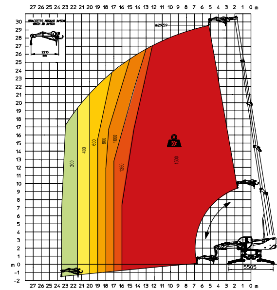
JW 1500 Jib winch 1.500 kg
