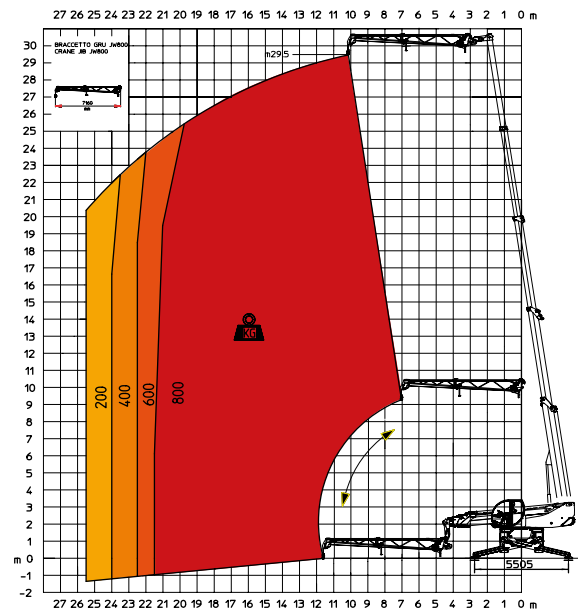
JW 800 Jib winch 800 kg
