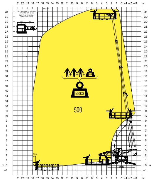
TP Telescopic Platform TP
