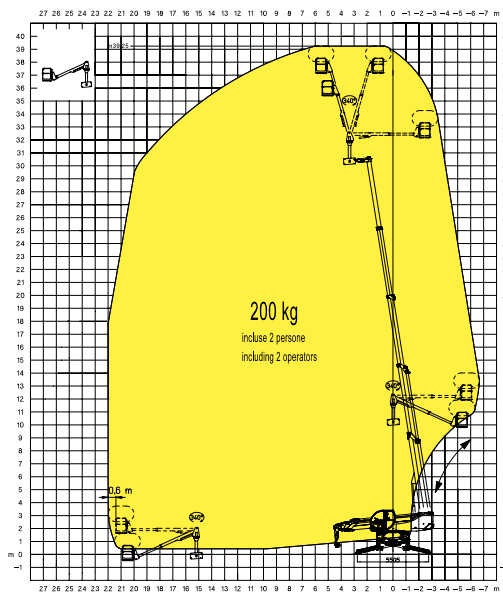
TP O-U Telescopic pivoting men platform over-under with 340° rotation
